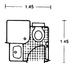
⑨ Bathroom cubicle
